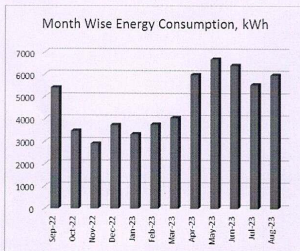
Figure 2.1 : Monthly Electrical Energy Consumption
